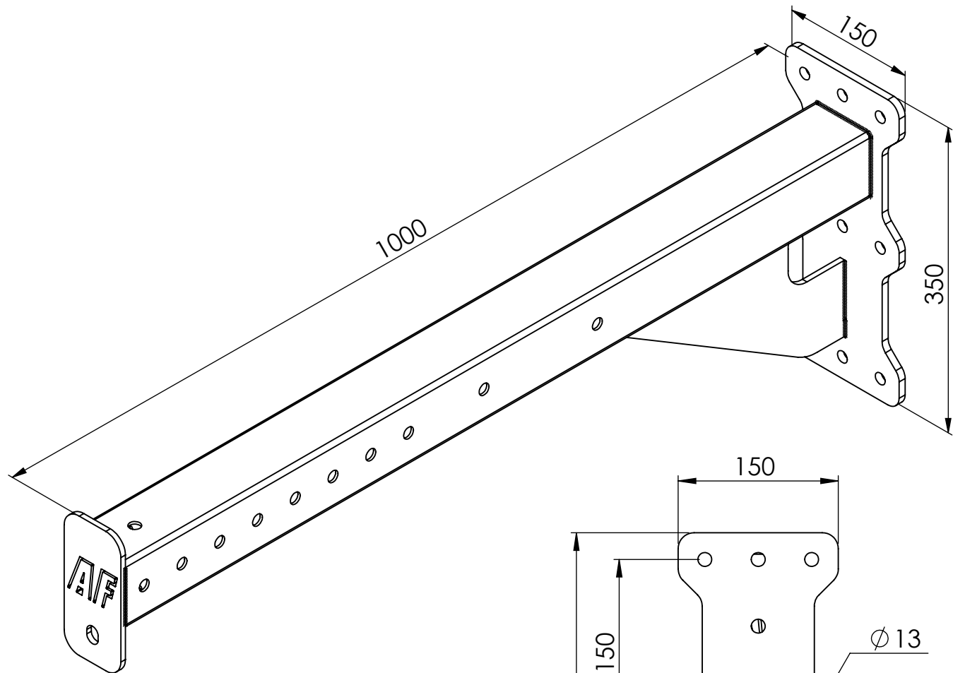
ISOMETRIC VIEW
